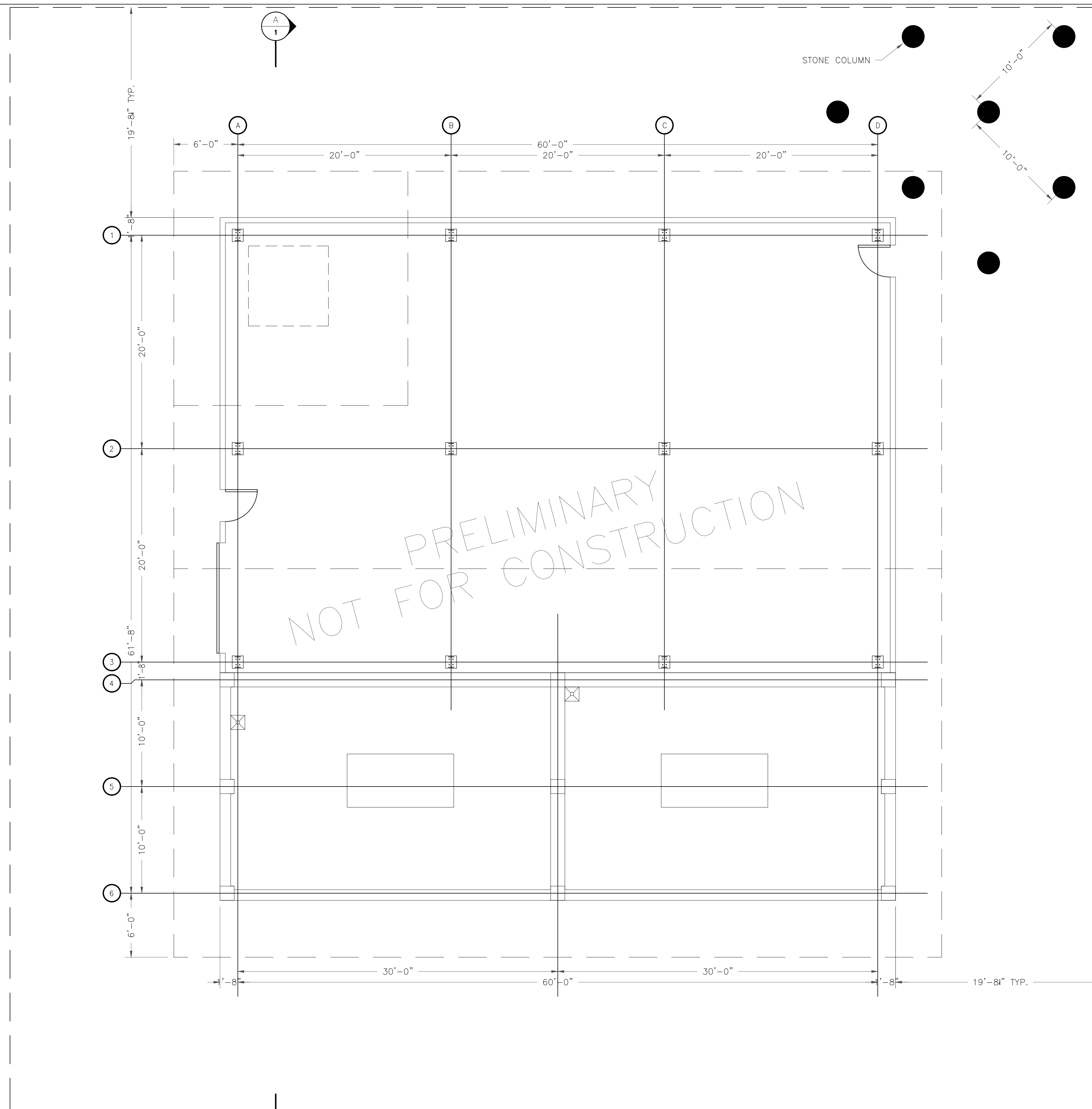
PLAN VIEW 3/16" = 1'-0"
