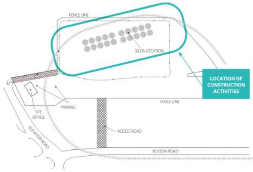
Grain bin remediation work area
